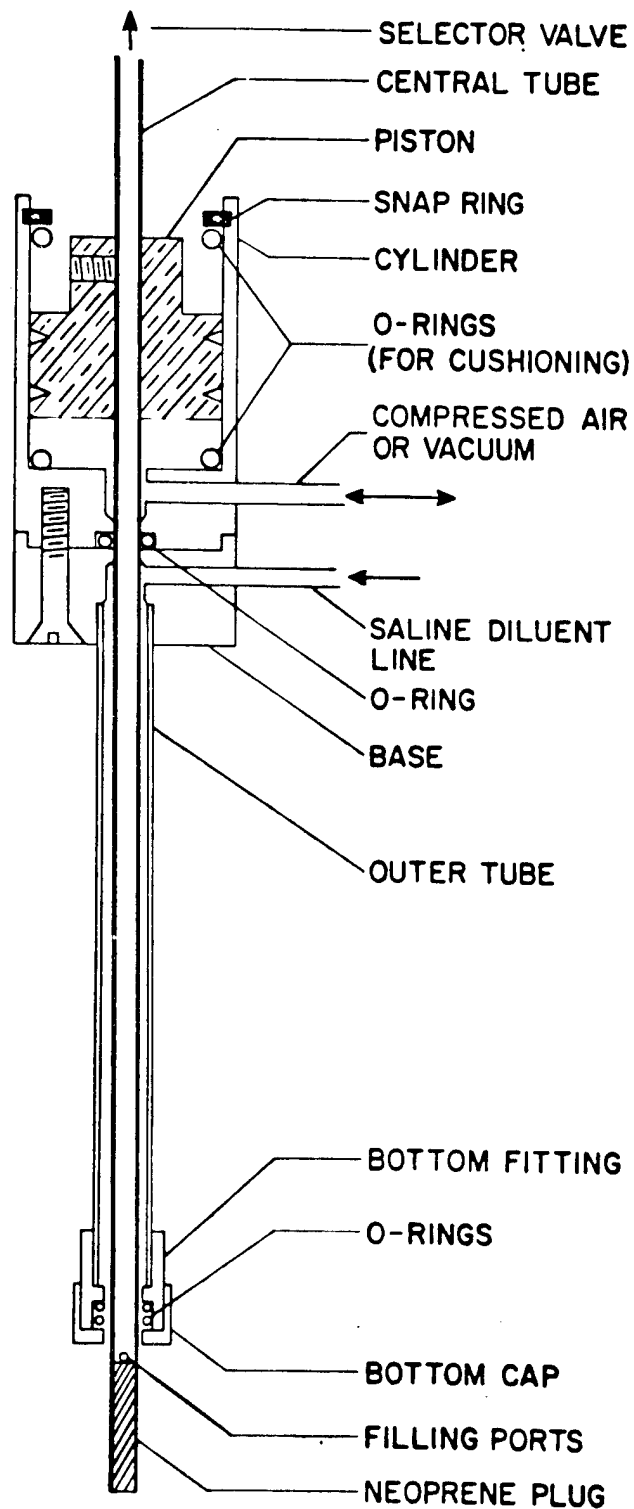
Fig. 2. Sampling valve.
